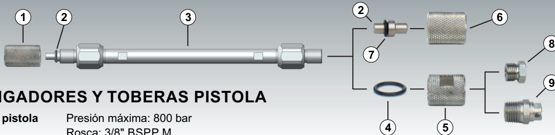
453244 BSPP 3/8" M 60°
